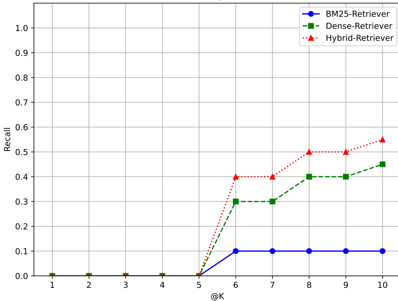
Query 17
